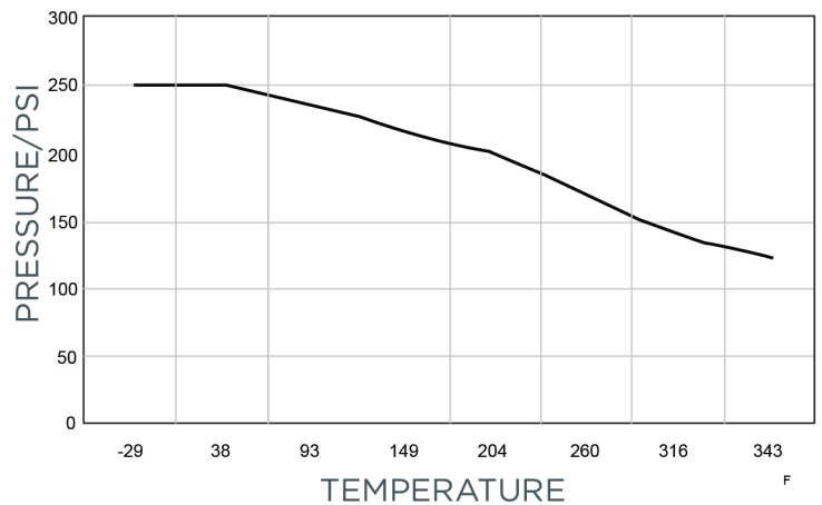
Pressure-temperature curve
